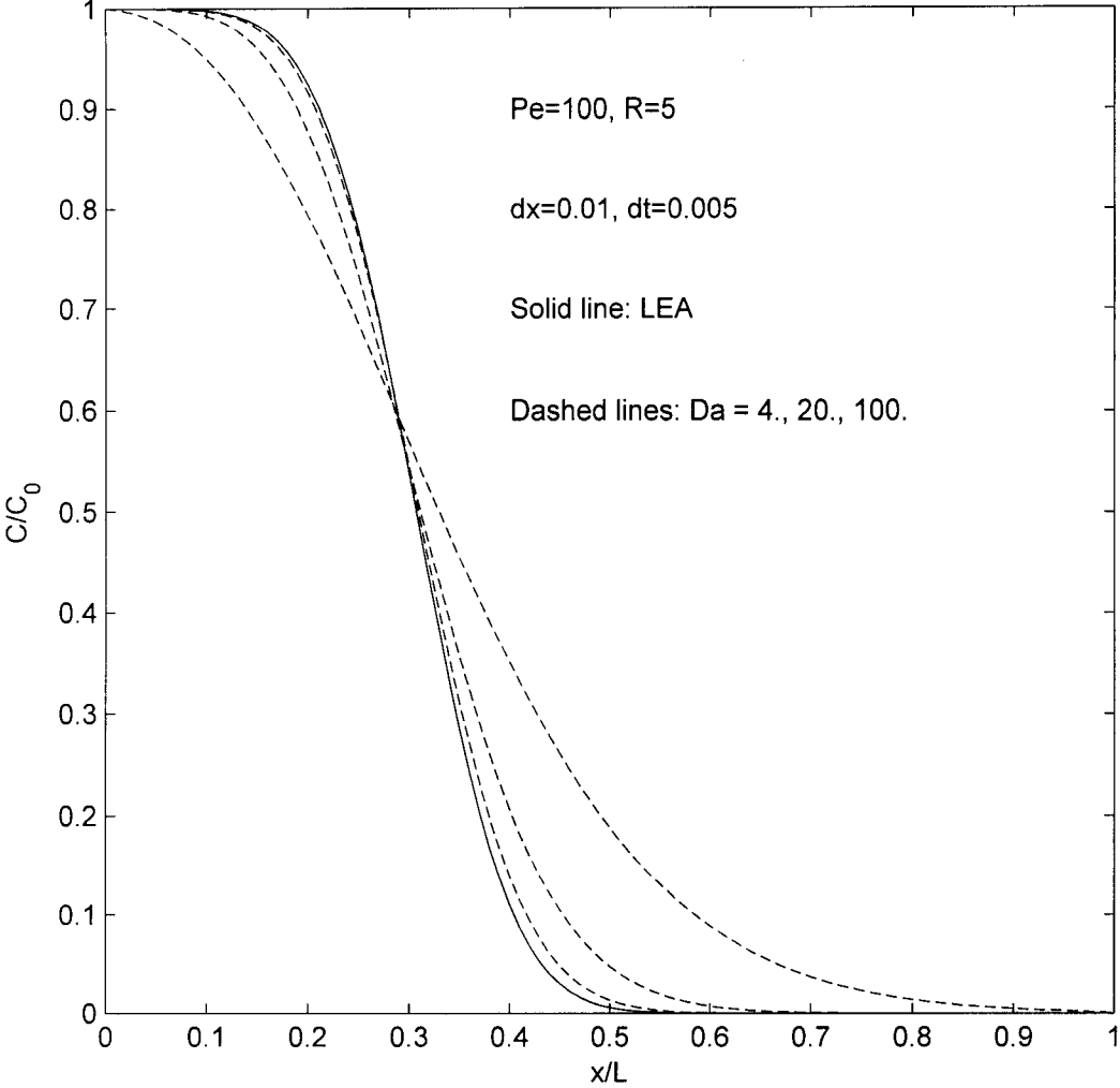
FEM model of transport with non-equilibrium sorption: Concentration profile at t = 0.3 \cdot R
