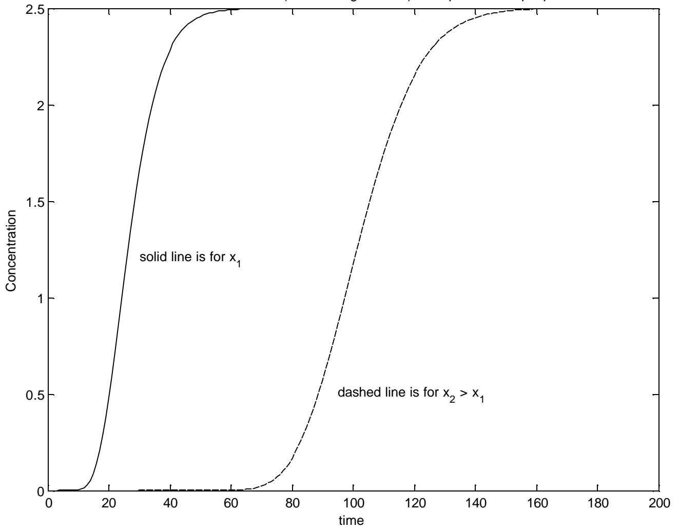
Concentration histories (breakthrough curves) in response to step input
