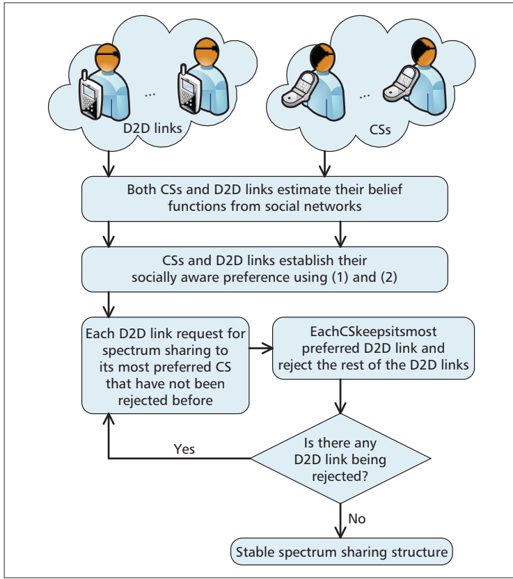
Figure 3. Algorithm for spectrum sharing between D2D links and CSs with social-awareness.
