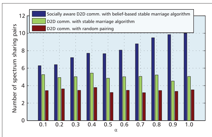
Figure 5. Number of spectrum sharing pairs formed between D2D links and CSs with and without social awareness.
