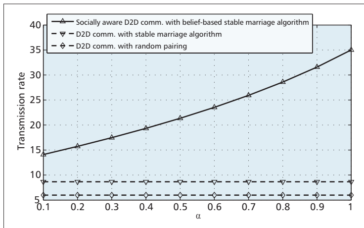
Figure 4. Spectrum utilization efficiency for D2D communication with social awareness.
