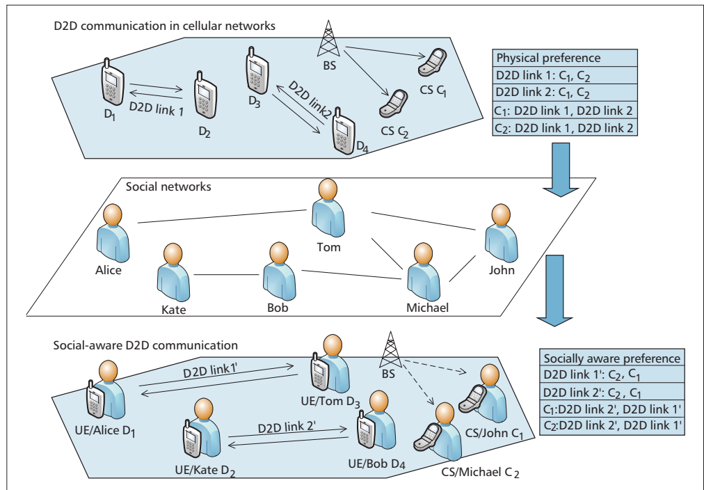
Figure 2. Illustration of socially aware preference for D2D communication with social awareness.
