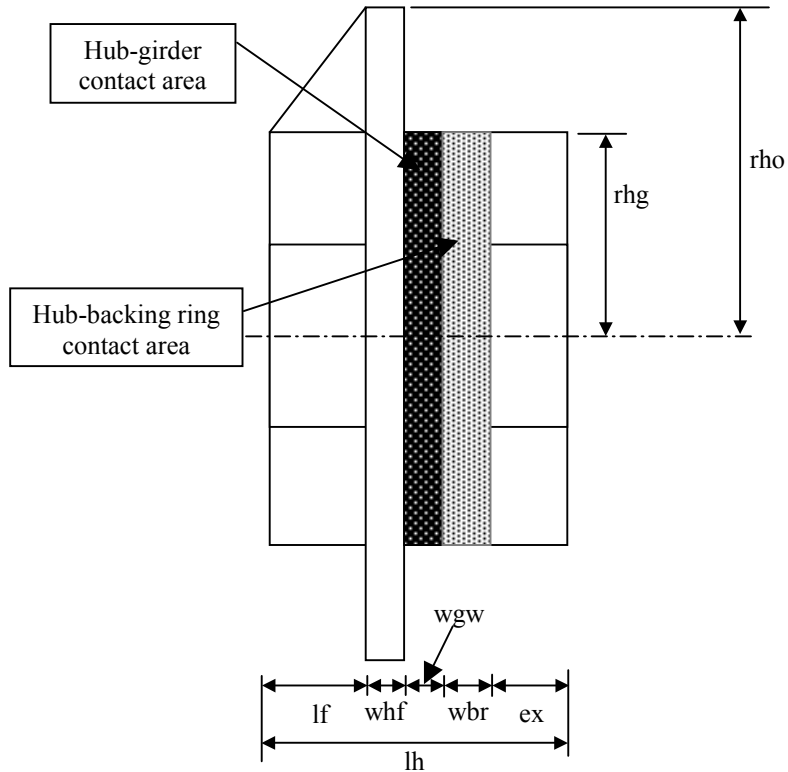
Figure B.14a Hub dimensions.
