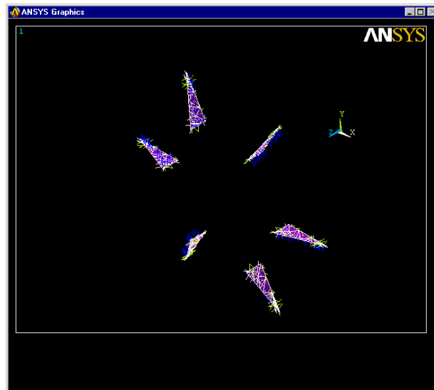
Figure 3.2b Thermal element SHELL57 and structural element SHELL63.
