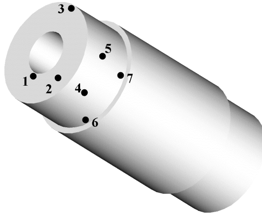
Figure 7.1 Gages on trunnion of AP1.
