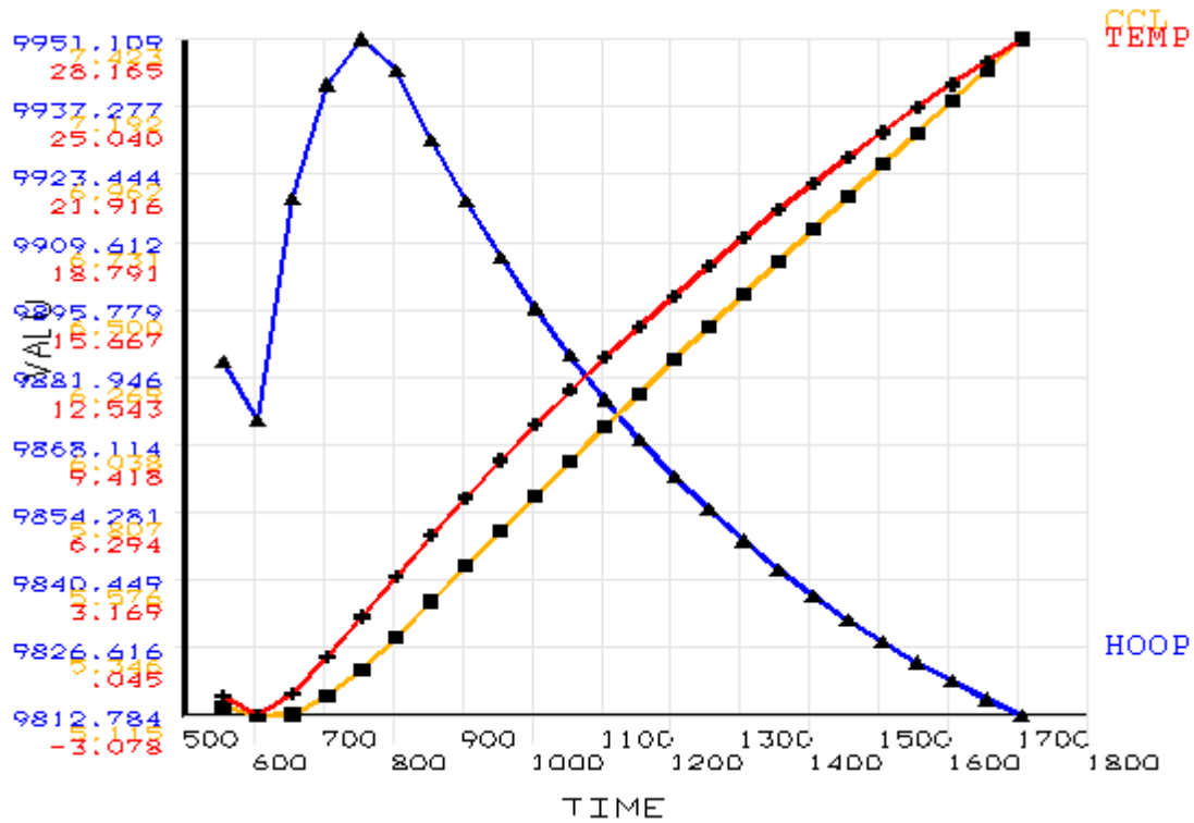
Figure 4.6 Critical parameters (CCL is critical crack length in inches, TEMP is temperature in ^{\circ}\text{F} , and HOOP is hoop stress in psi) plotted against time (sliding the trunnion-hub assembly into the girder during AP1 of Christa McAuliffe Bridge).
