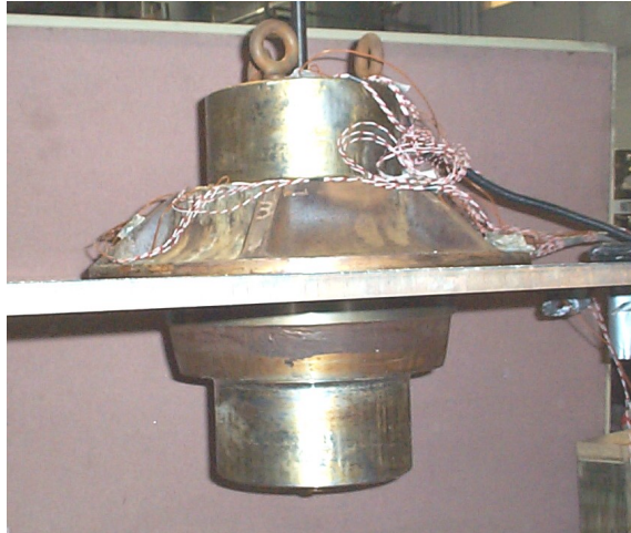
Figure 7.28 THG assembly lifted by the overhead crane.
