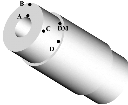
Figure 6.2 Positions of gages on quarter-scale trunnion.
