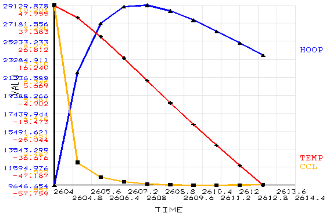
Figure 4.29b Critical parameters (CCL is critical crack length in inches, TEMP is temperature in °F, and HOOP is hoop stress in psi) plotted against time (cooling down of the trunnion-hub assembly during AP1 of the Hillsborough Avenue Bridge).
