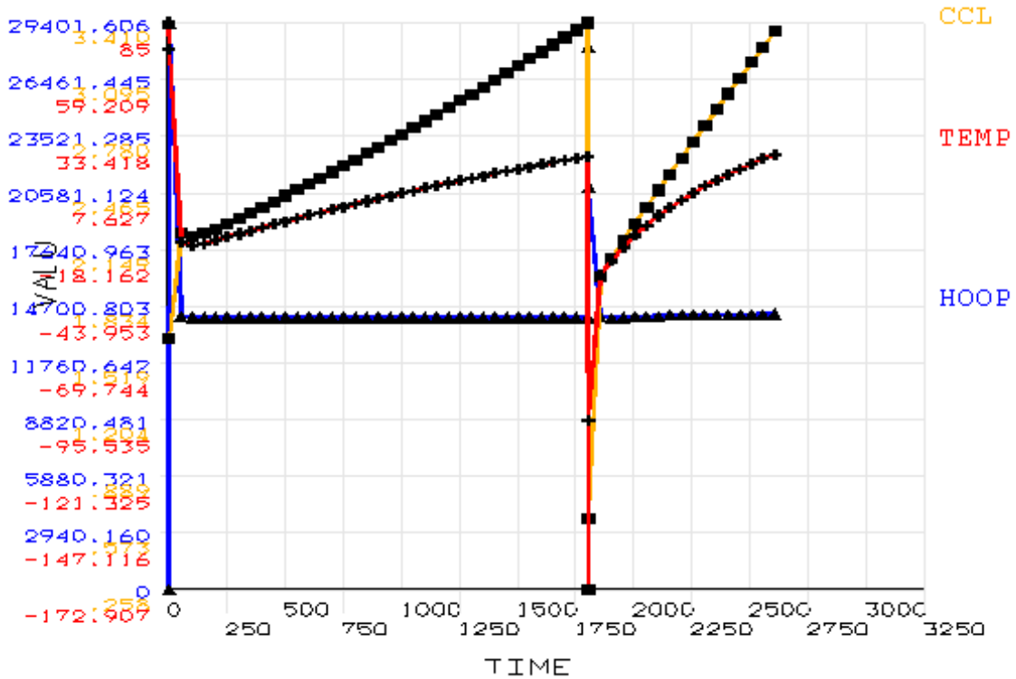
Figure 4.21 Critical parameters (CCL is critical crack length in inches, TEMP is temperature in ^{\circ}\text{F} , and HOOP is hoop stress in psi) plotted against time (full assembly process during AP1 of 17 th Street Causeway Bridge).
