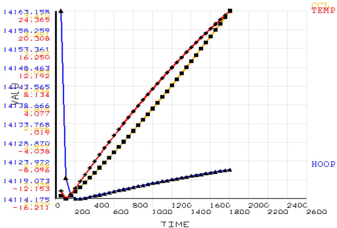
Figure 4.22 Critical parameters (CCL is critical crack length in inches, TEMP is temperature in 0 F, and HOOP is hoop stress in psi) plotted against time (sliding the trunnion into the hub during AP1 of 17 th Street Causeway Bridge).
