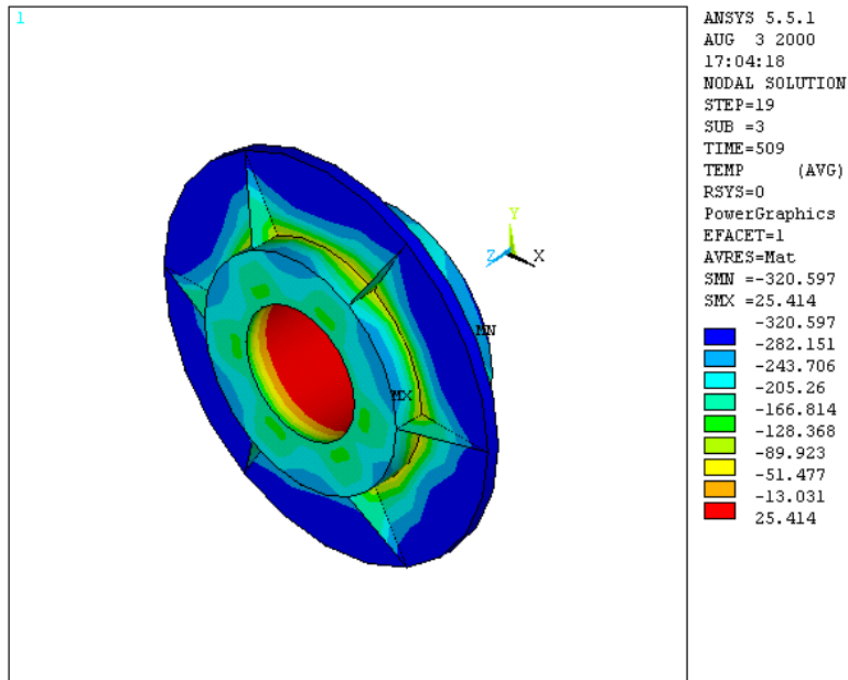
Figure 4.5e Temperature (°F) plot when the lowest critical crack length during AP1 is observed.
