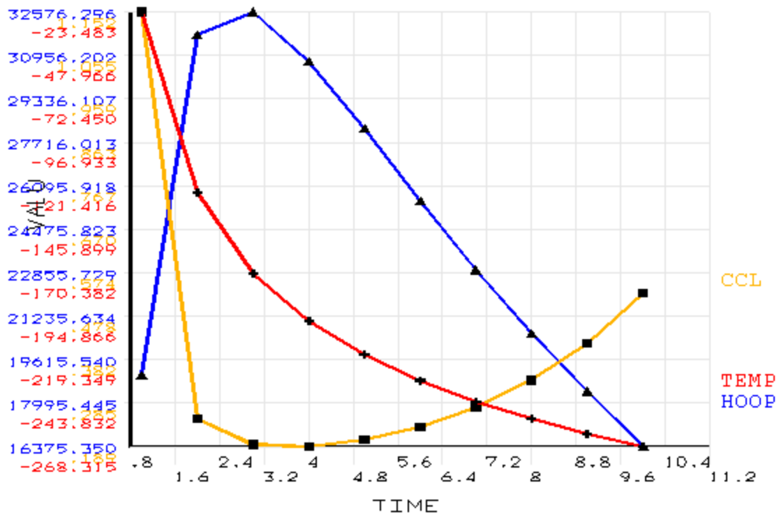
Figure 4.17 Critical parameters (CCL is critical crack length in inches, TEMP is temperature in °F, and HOOP is hoop stress in psi) plotted against time (cooling down of the hub during AP2 of the Hillsborough Avenue Bridge).
