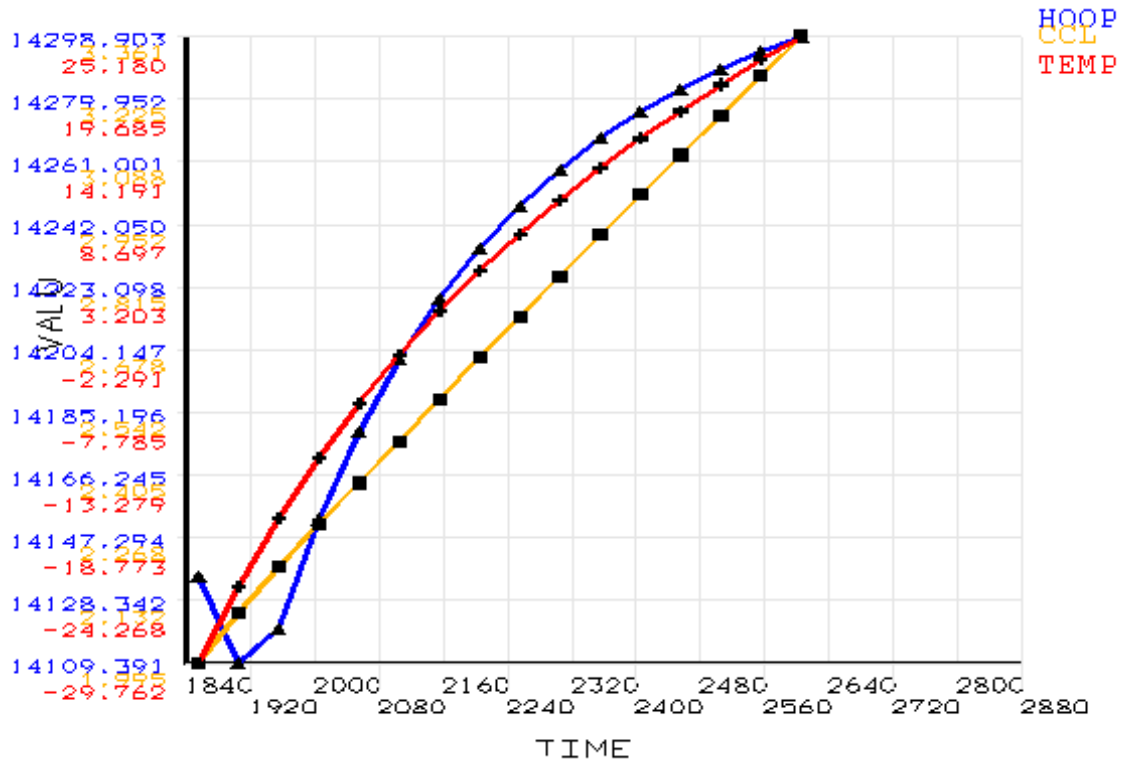
Figure 4.24 Critical parameters (CCL is critical crack length in inches, TEMP is temperature in 0 F, and HOOP is hoop stress in psi) plotted against time (sliding the trunnion-hub assembly into the girder during AP1 of the 17 th Street Causeway Bridge).
