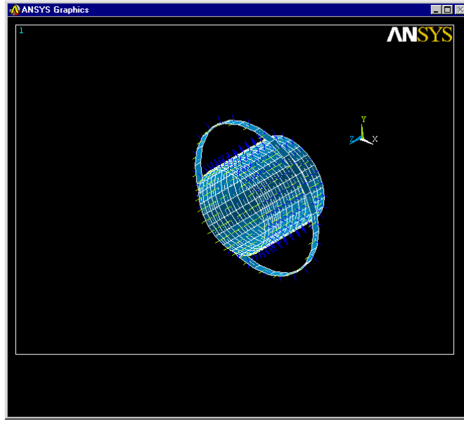
Figure 3.2c Contact elements CONTACT174 and TARGET170.
