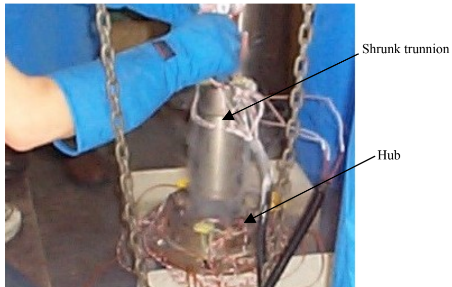
Figure 6.1 Cooled trunnion being inserted into the hub.
