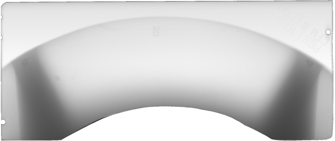
Figure D.2e X-ray of the hub from the web view (4-5).
