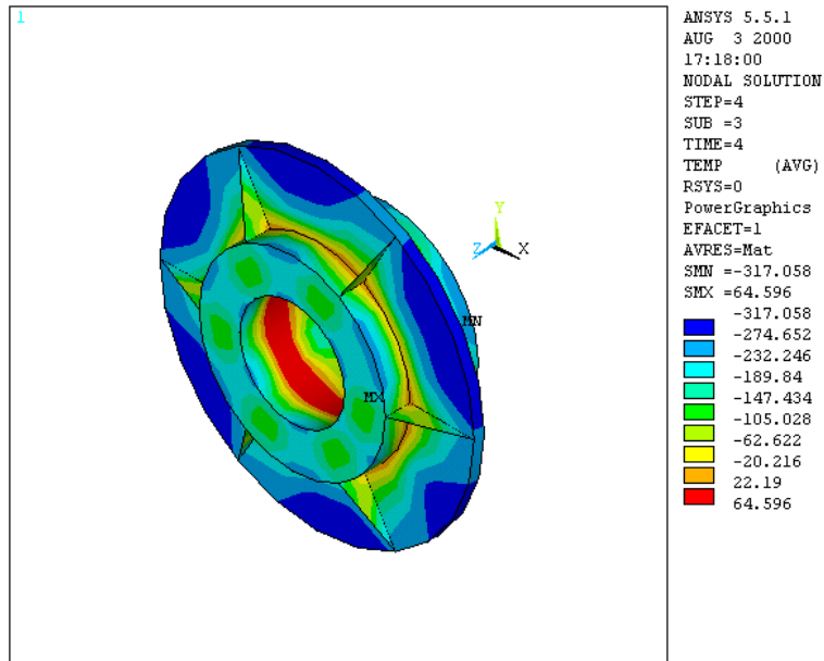
Figure 4.8e Temperature ( ^{\circ} F) plot when the lowest critical crack length during AP2 is observed.
