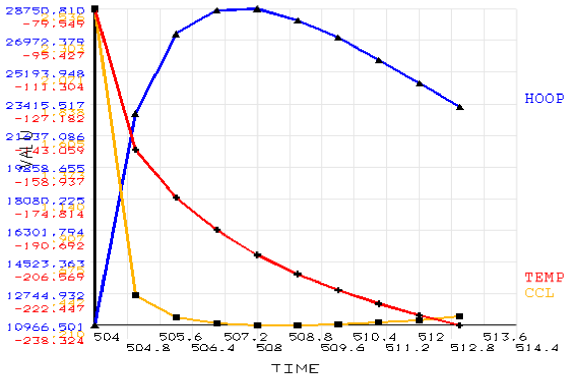
Figure 4.5a Critical parameters (CCL is critical crack length in inches, TEMP is temperature in °F, and HOOP is hoop stress in psi) plotted against time (cooling down of the trunnion-hub assembly during AP1 of the Christa McAuliffe Bridge).
