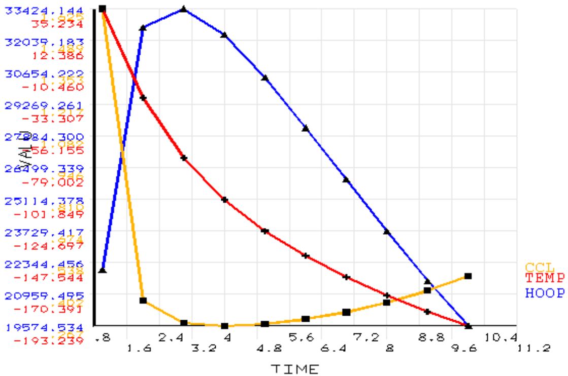
Figure 4.8a Critical parameters (CCL is critical crack length in inches, TEMP is temperature in 0 F, and HOOP is hoop stress in psi) plotted against time (cooling down of the hub during AP2 of the Christa McAuliffe Bridge).
