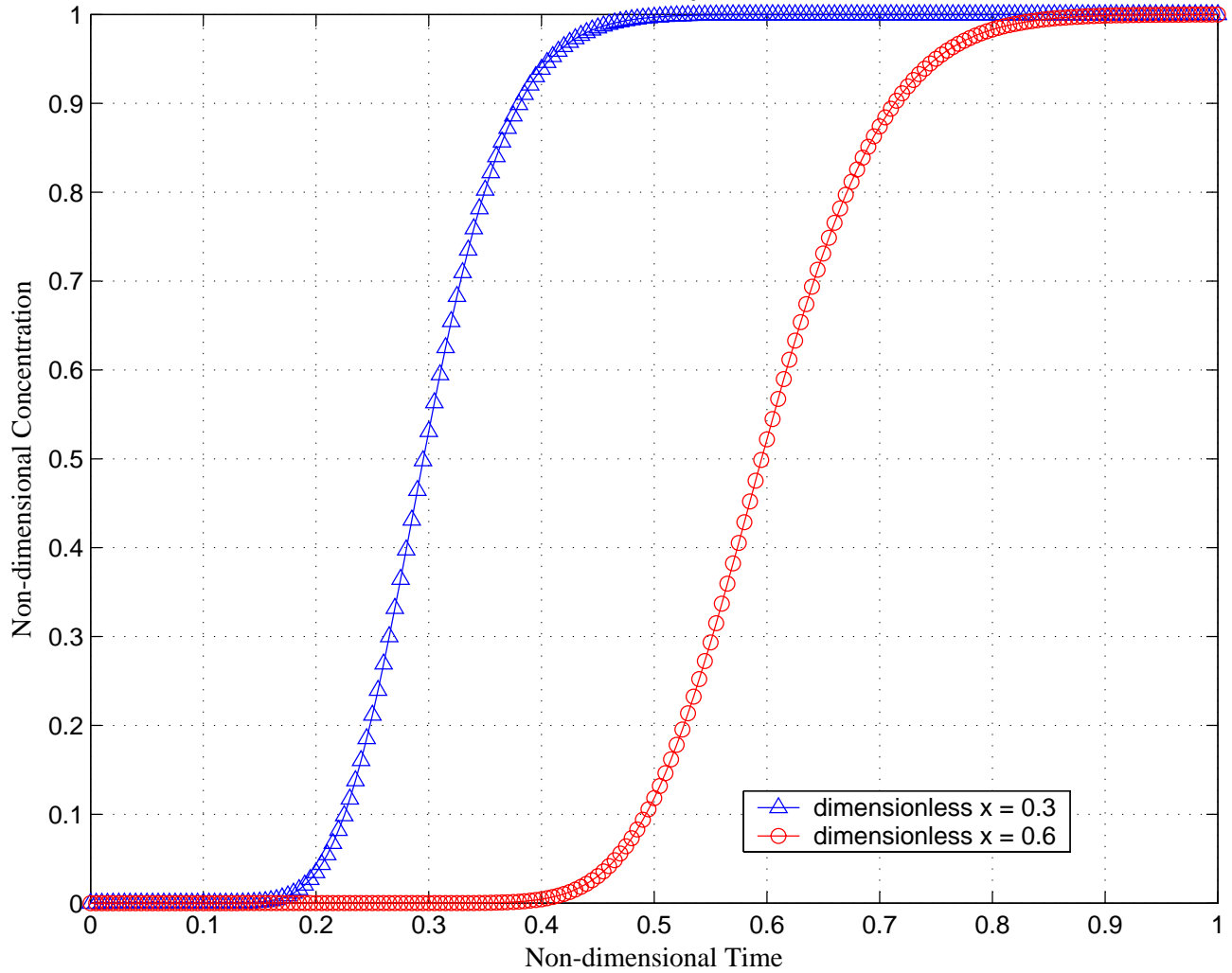
Concentration history with Pe = 160
