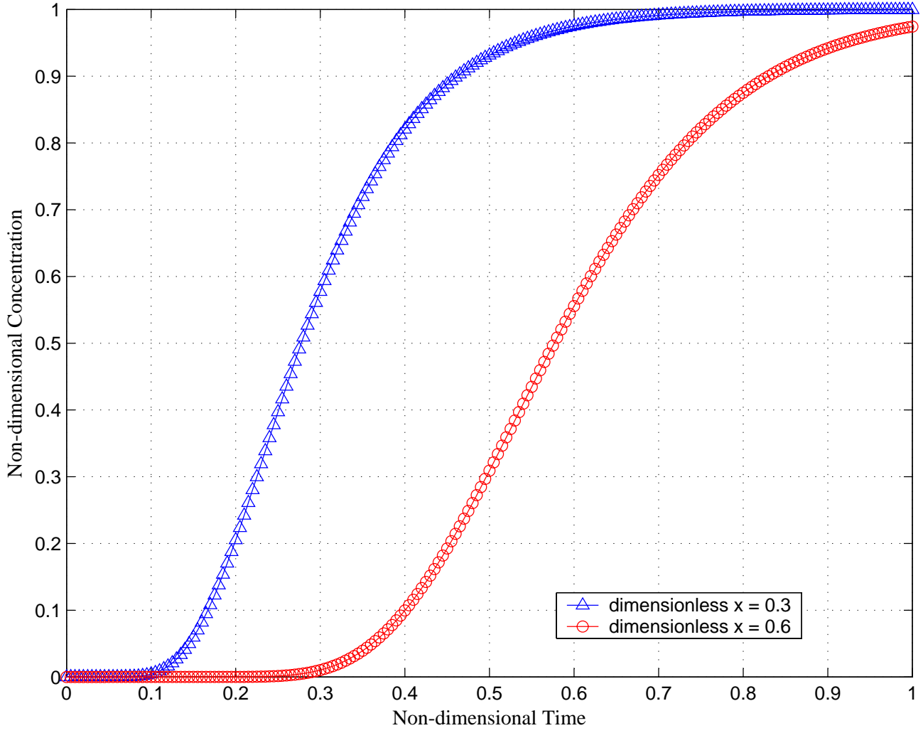
Concentration history with Pe = 40
