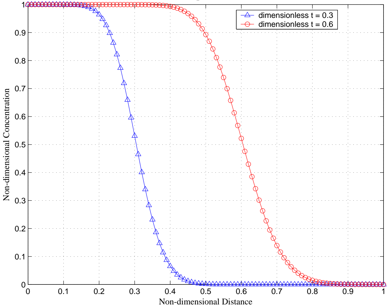
Concentration profile with Pe=160
