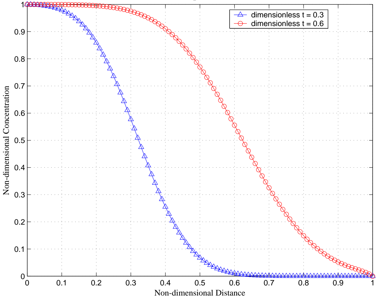
Concentration profile with Pe=40
