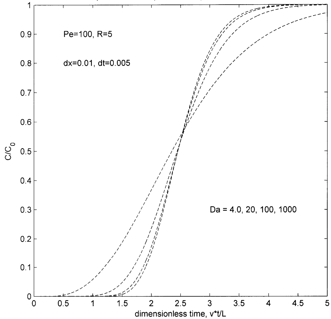
FEM model of transport with non-equilibrium sorption: Concentration history at x = L/2
