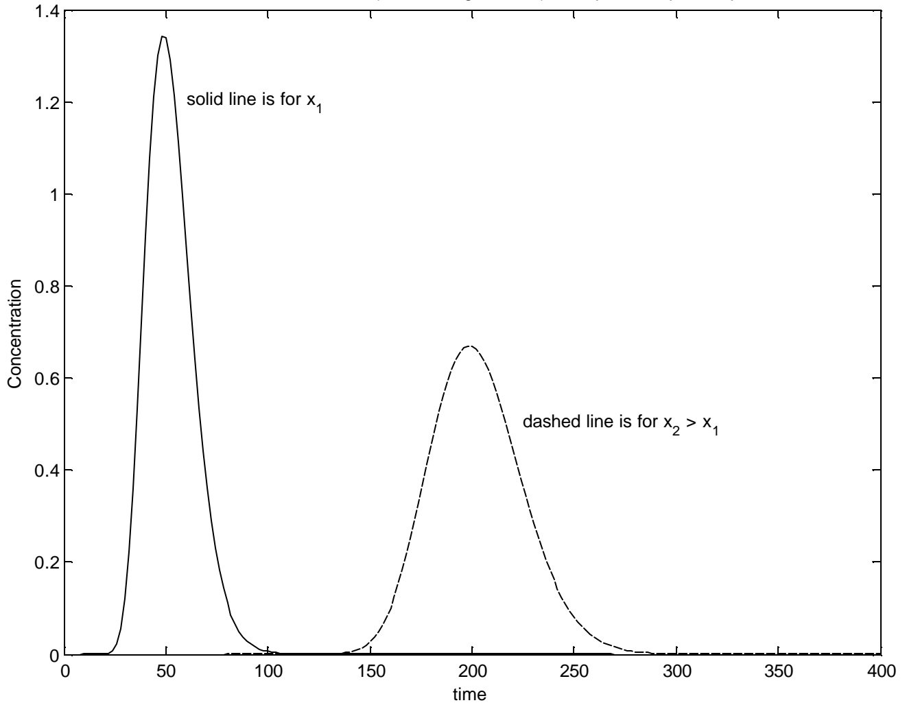
Concentration histories (breakthrough curves) in response to pulse input
